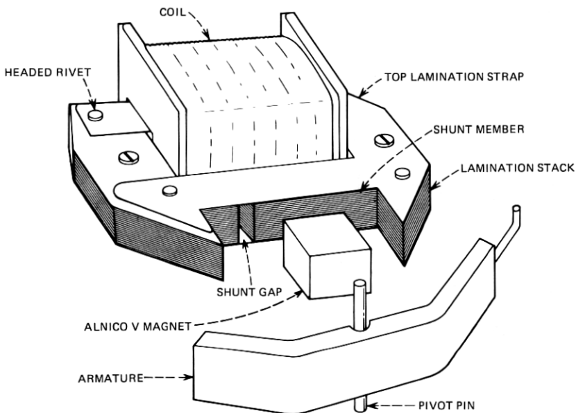
Fig. 2—Rocking-armature motor.
