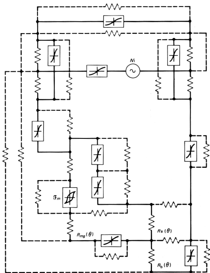
Fig. 14—Lumped element model of P-ringer motor.
